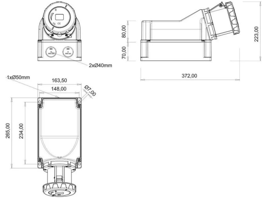
TECHNICAL DRAWING
