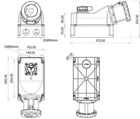
TECHNICAL DRAWING
