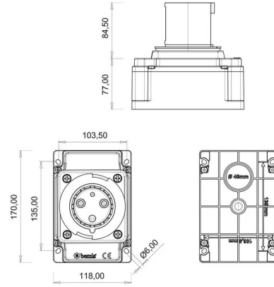
TECHNICAL DRAWING
