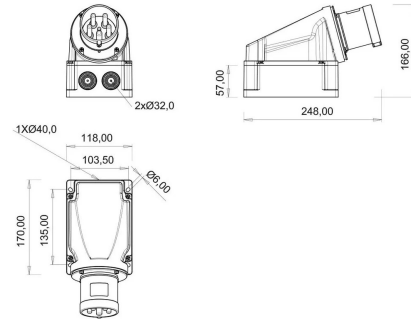
TECHNICAL DRAWING
