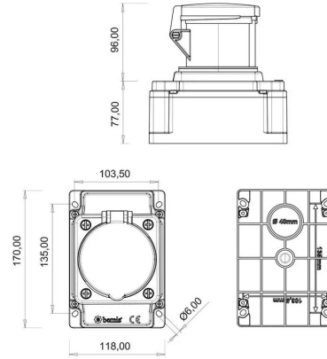
TECHNICAL DRAWING
