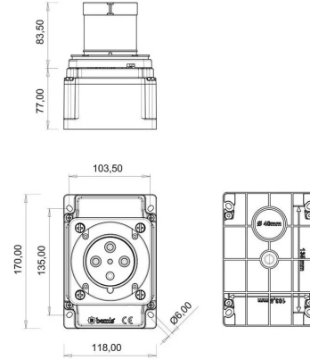
TECHNICAL DRAWING
