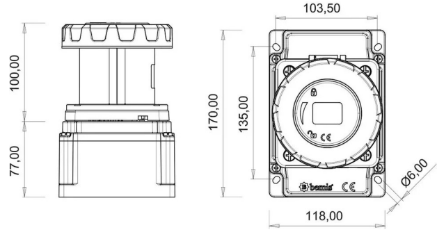
TECHNICAL DRAWING
