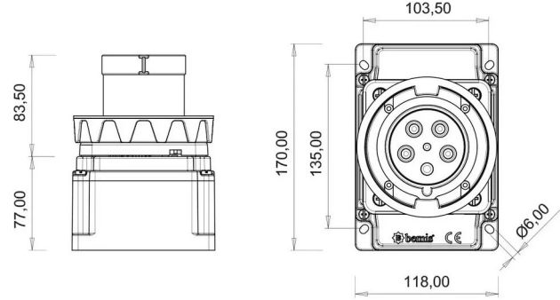
TECHNICAL DRAWING
