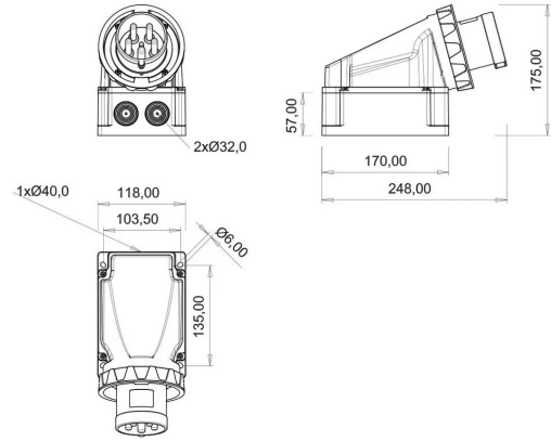
TECHNICAL DRAWING
