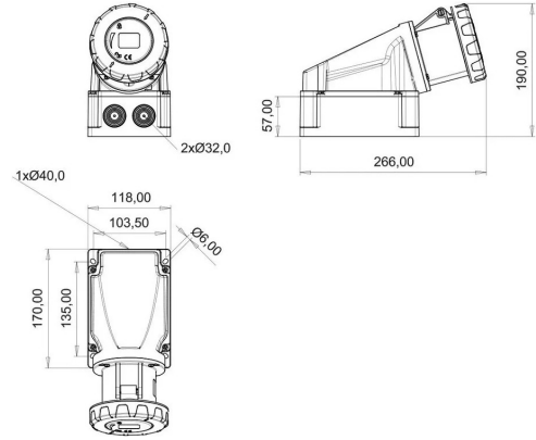
TECHNICAL DRAWING
