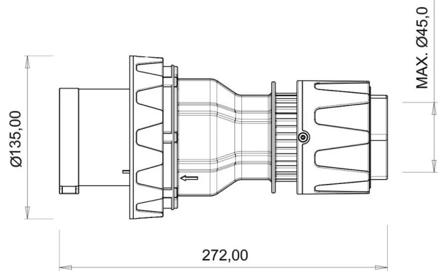
TECHNICAL DRAWING
