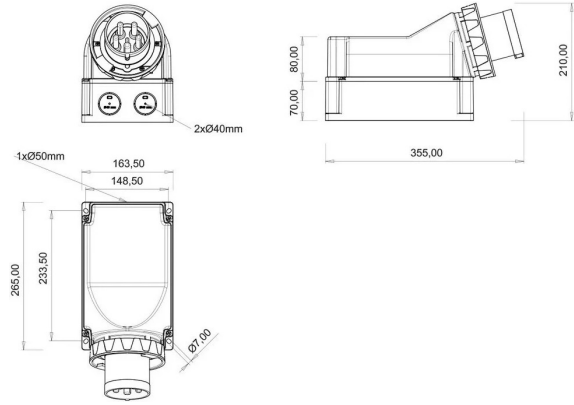
TECHNICAL DRAWING
