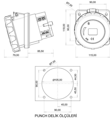
TECHNICAL DRAWING
