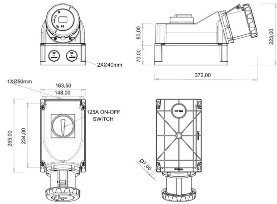
TECHNICAL DRAWING
