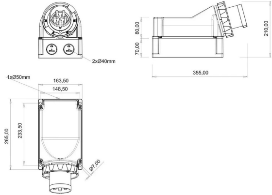
TECHNICAL DRAWING
