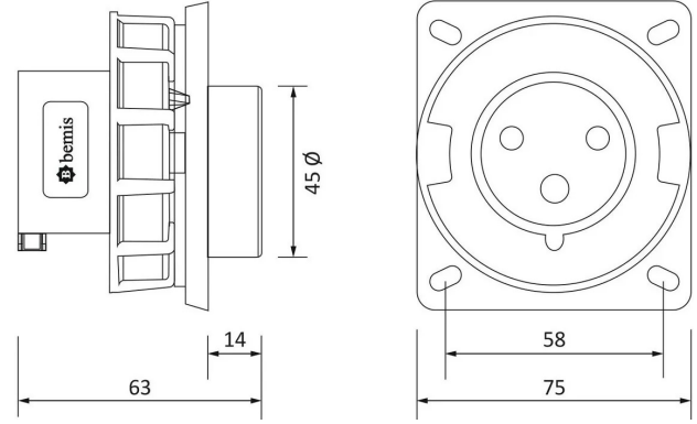
TECHNICAL DRAWING
