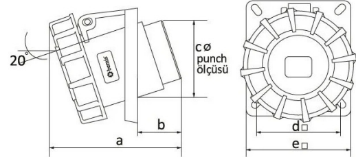
TECHNICAL DRAWING
