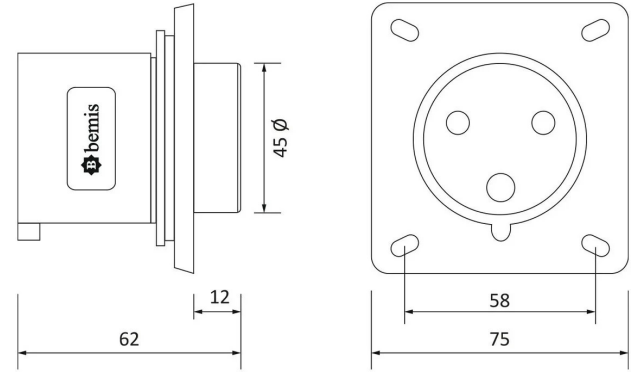
TECHNICAL DRAWING
