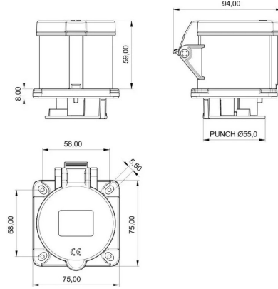
TECHNICAL DRAWING
