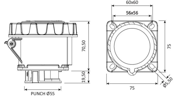
TECHNICAL DRAWING
