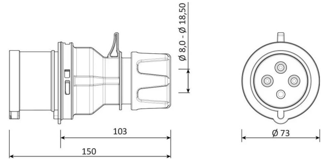
TECHNICAL DRAWING
