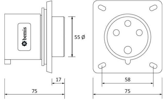
TECHNICAL DRAWING
