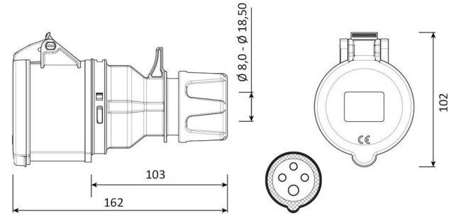
TECHNICAL DRAWING
