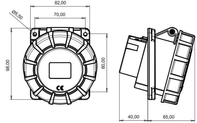
TECHNICAL DRAWING
