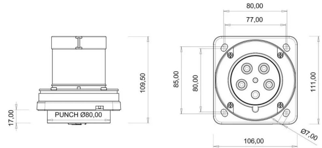
TECHNICAL DRAWING
