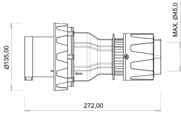
TECHNICAL DRAWING
