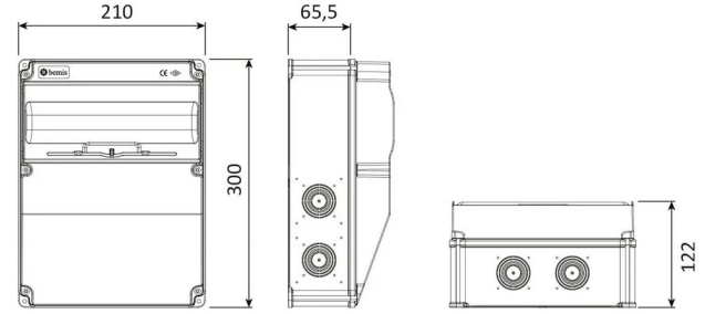
TECHNICAL DRAWING
