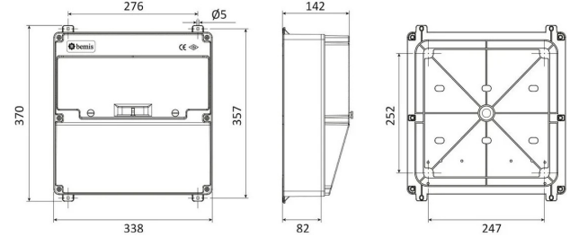
TECHNICAL DRAWING
