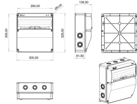
TECHNICAL DRAWING
