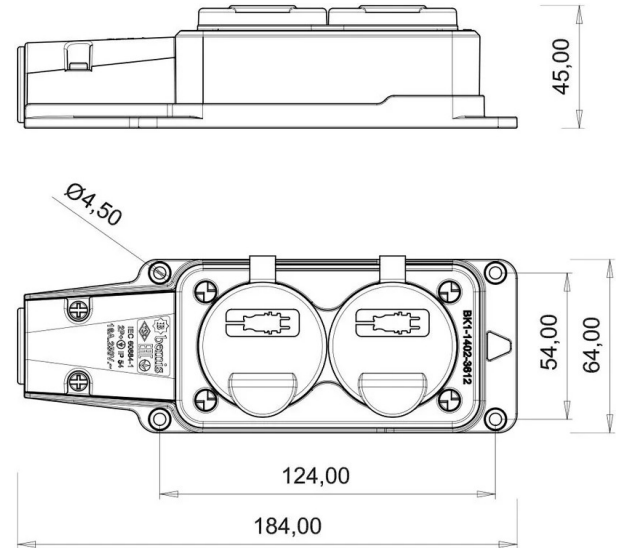
TECHNICAL DRAWING
