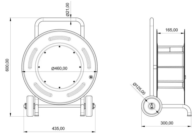
TECHNICAL DRAWING
