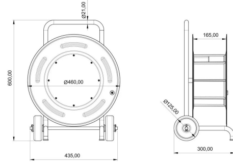
TECHNICAL DRAWING
