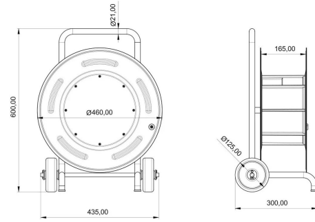
TECHNICAL DRAWING
