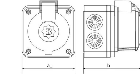
TECHNICAL DRAWING
