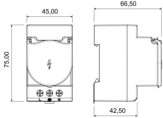
TECHNICAL DRAWING
