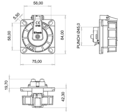
TECHNICAL DRAWING
